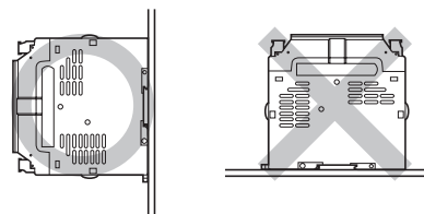
Standardmontage
